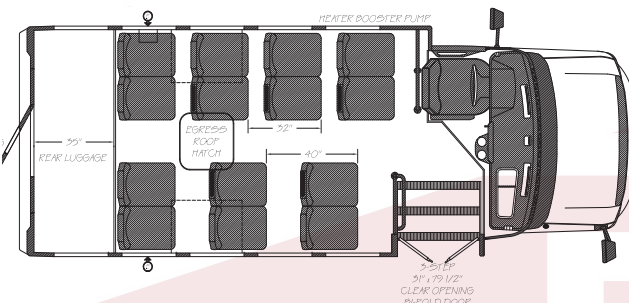
VIP 2200 - 14 PASS & REAR LUGG.
