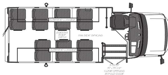
VIP 2200 - 14 PASS & REAR LUGG.
